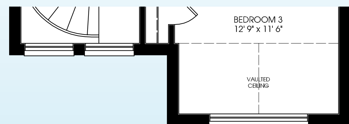
SECOND FLOOR - ELEV. A
