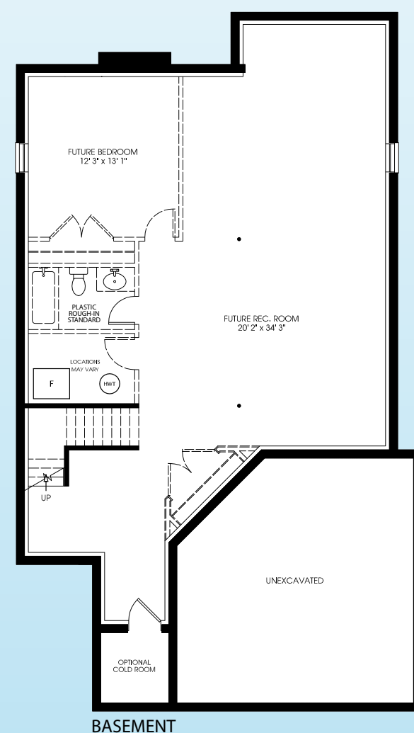
BASEMENT
